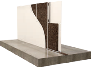
Internal partitions Metal-stud wall and slab discontinuity
